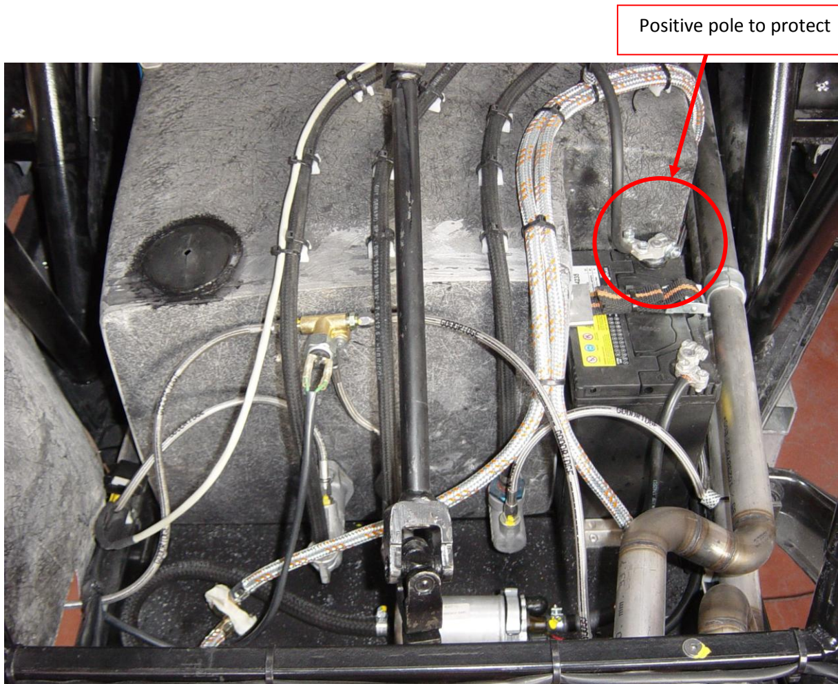
Figure 5: Good fixation of the wiring and pipes in the neighborhood of the battery
